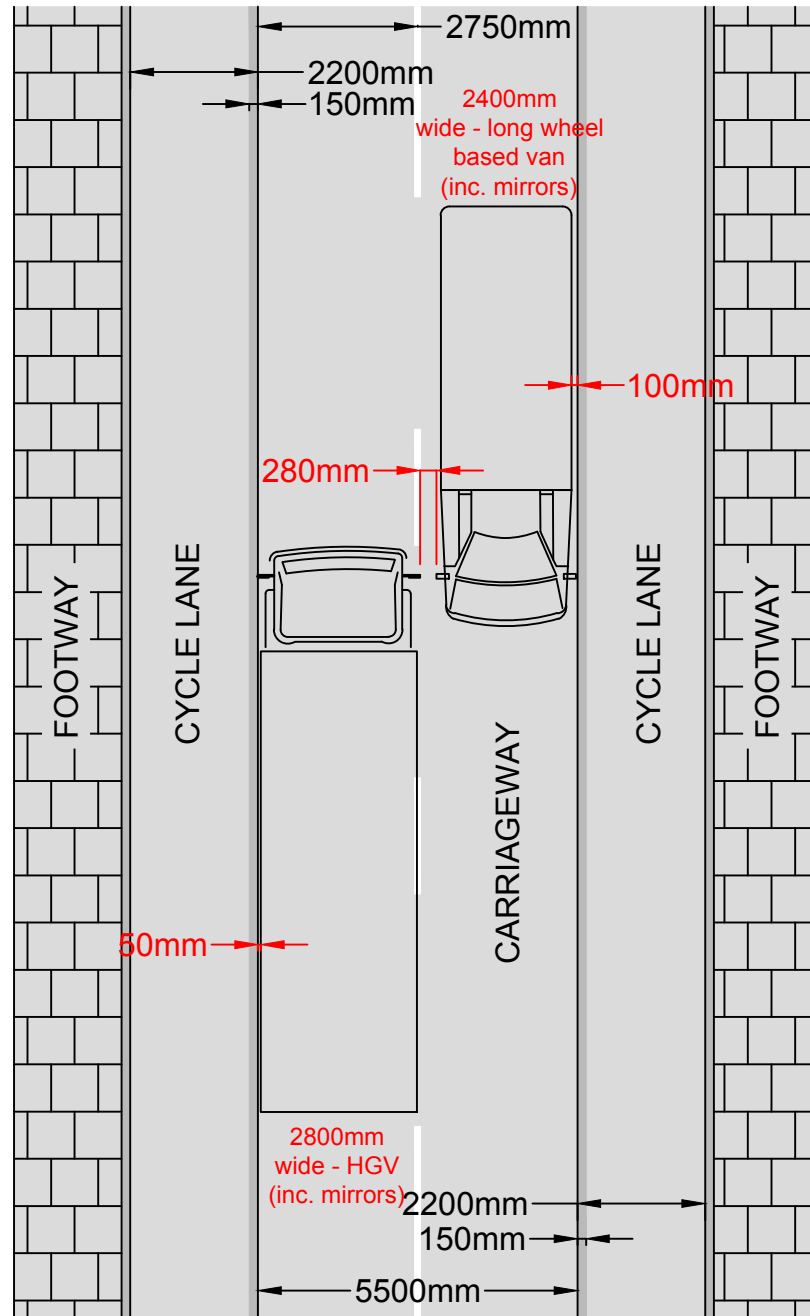
HGV vs LONG WHEEL BASED VAN
