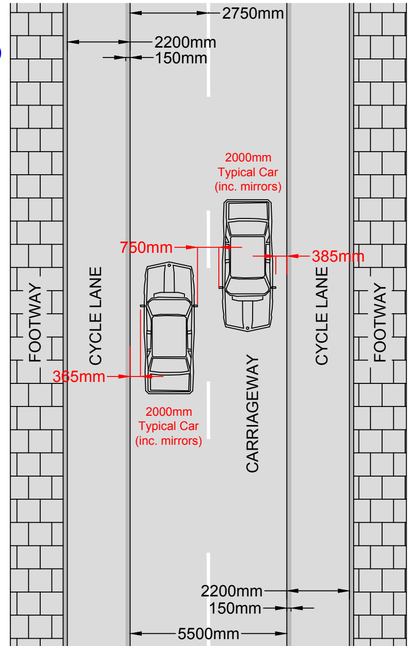
STANDARD CAR vs STANDAR CAR
