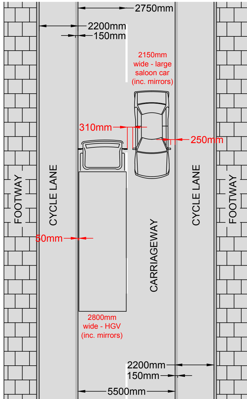
HGV vs LARGE SALOON CAR
